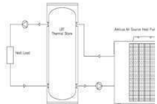
Amicus HT providing heating only
